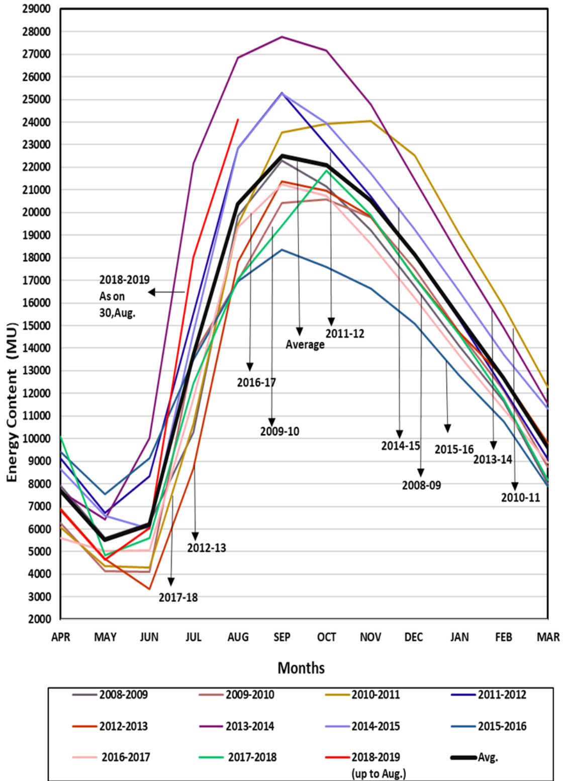
Month-wise Energy Content in Reservoir based H.E. Stations (MU)
