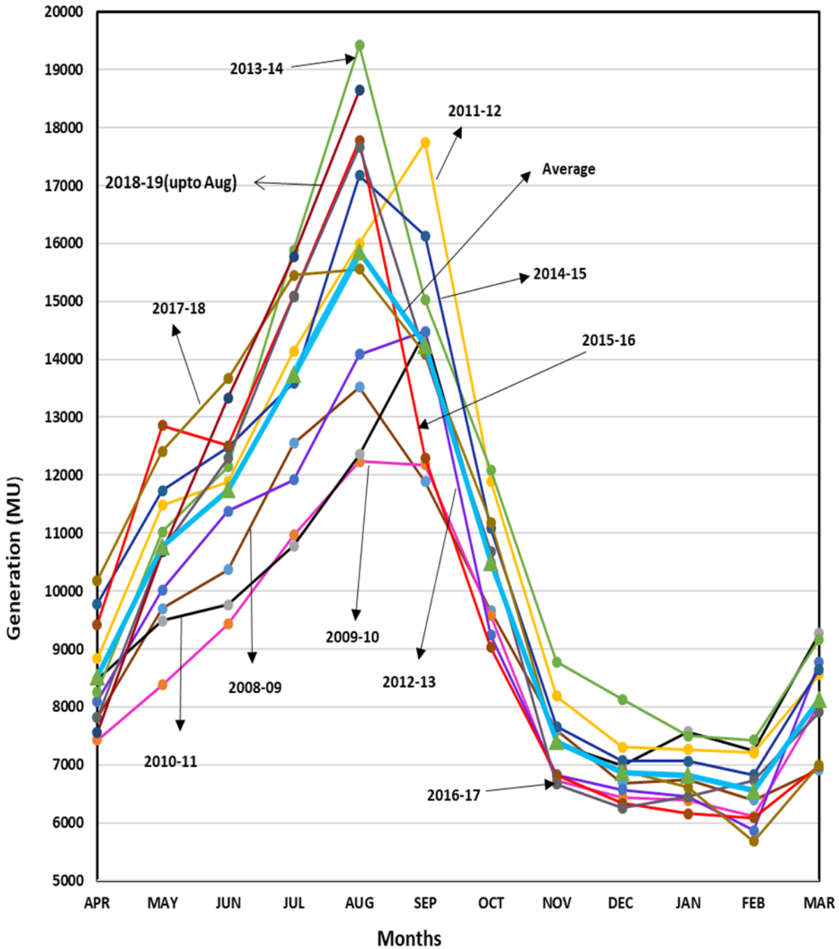
Month-wise Overall Energy Generation Pattern of H.E. Stations (MU)
